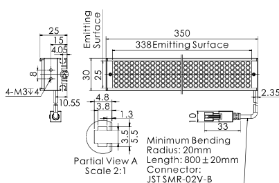
19.OPT-LI35030
